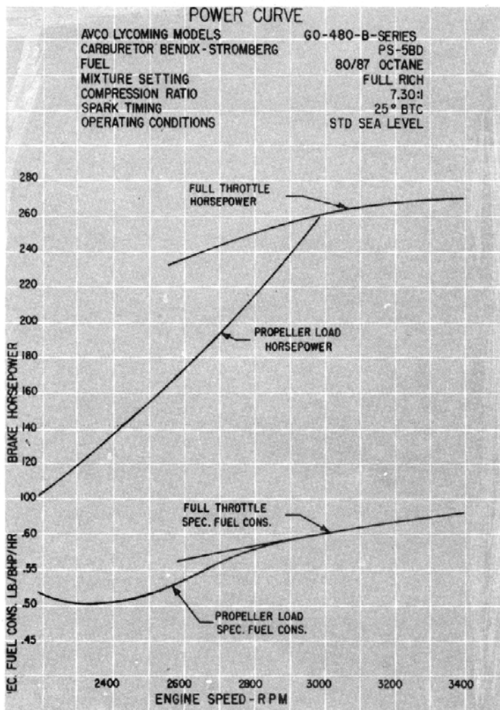
Figure 3-3. Sea Level Power Curve - GO-480-B Series
