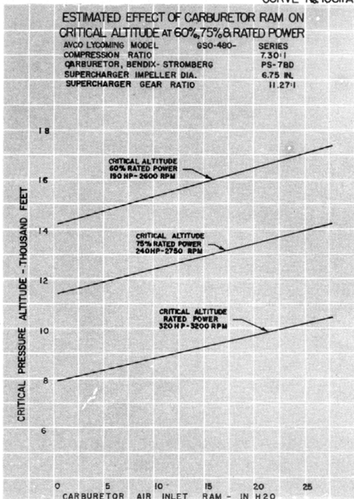
Figure 3-18. Estimated Effect of Carburetor Ram on Critical Altitude - GSO-480 Series
