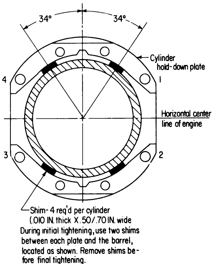
Figure 5-2. Location of Shims Between Cylinder Barrel and Hold-Down Plates (where applicable) and Sequence of Tightening Cylinder Base Hold-Down Nuts
