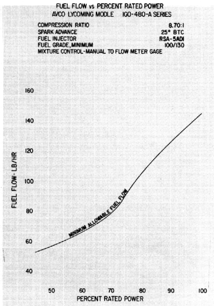
Figure 3-26. Fuel Flow vs Percent Rated Power - IGO-480-A Series
