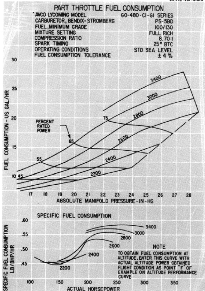
Figure 3-5. Part Throttle Fuel Consumption Curve - GO-480-C1, -G1 Series
