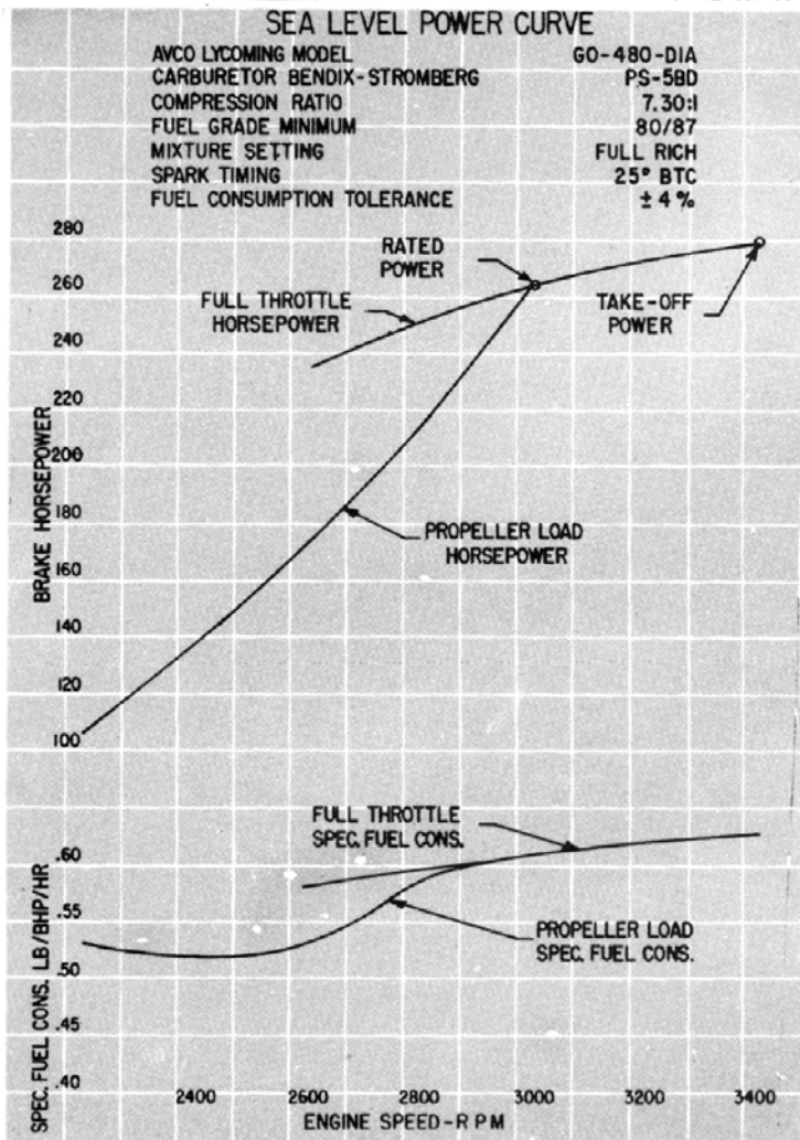
Figure 3-12. Sea Level Power Curve - GO-480-D Series
