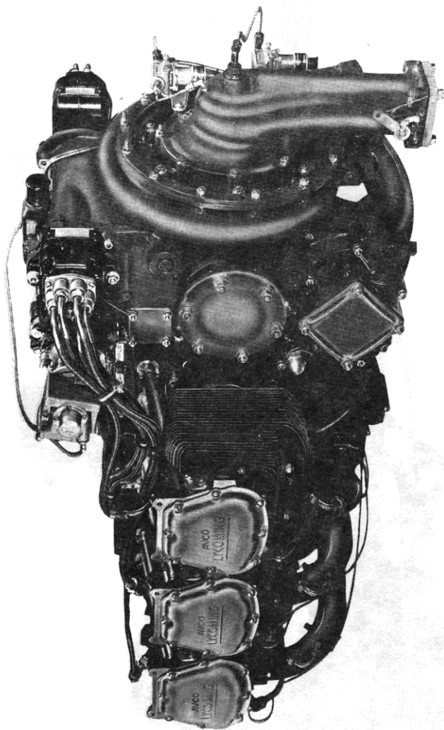
3/4 Rear View - IGSO-480
