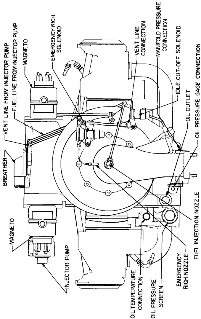
Figure 7-5. Rear View, IGSO-480 - Simmonds Injector
