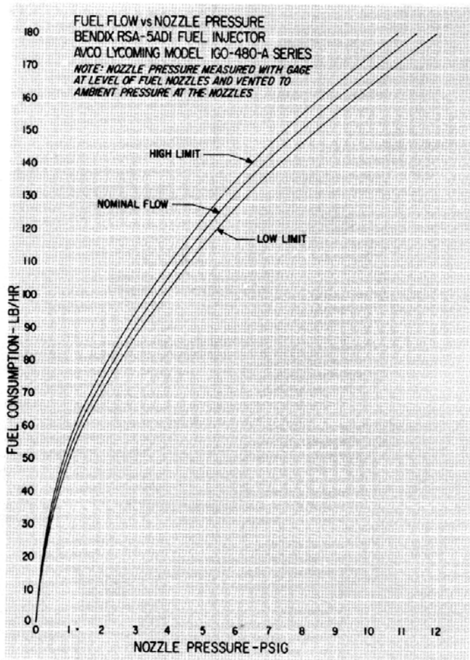
Figure 3-25. Fuel Flow vs Nozzle Pressure - IGO-480-A Series
