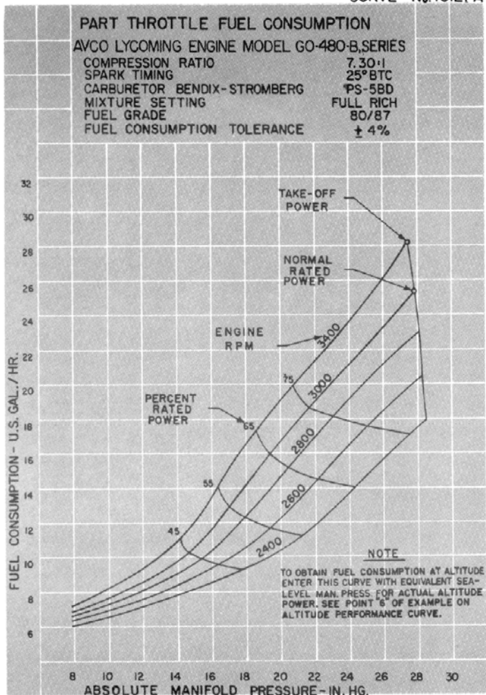
Figure 3-2. Part Throttle Fuel Consumption Curve - GO-480-B Series
