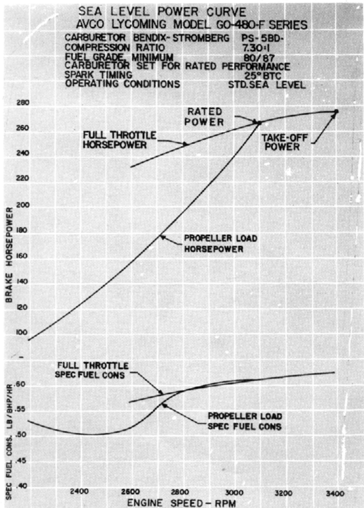
Figure 3-15. Sea Level Power Curve - GO-480-F Series
