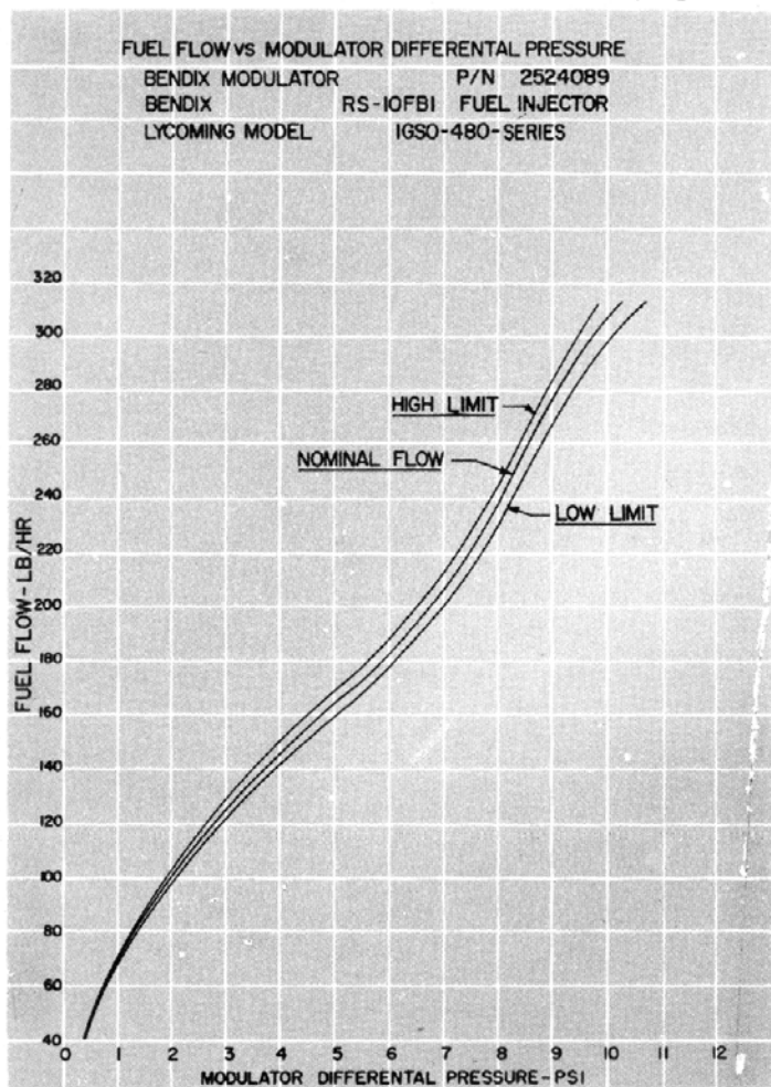
Figure 3-22. Fuel Flow vs Modulator Differential Pressure - IGSO-480-A1D6, -A1E6, -A1G6
