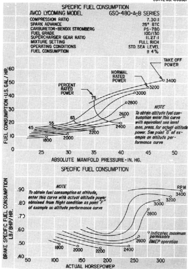
Figure 3-17. Specific Fuel Consumption - GSO-480-A, -B Series
