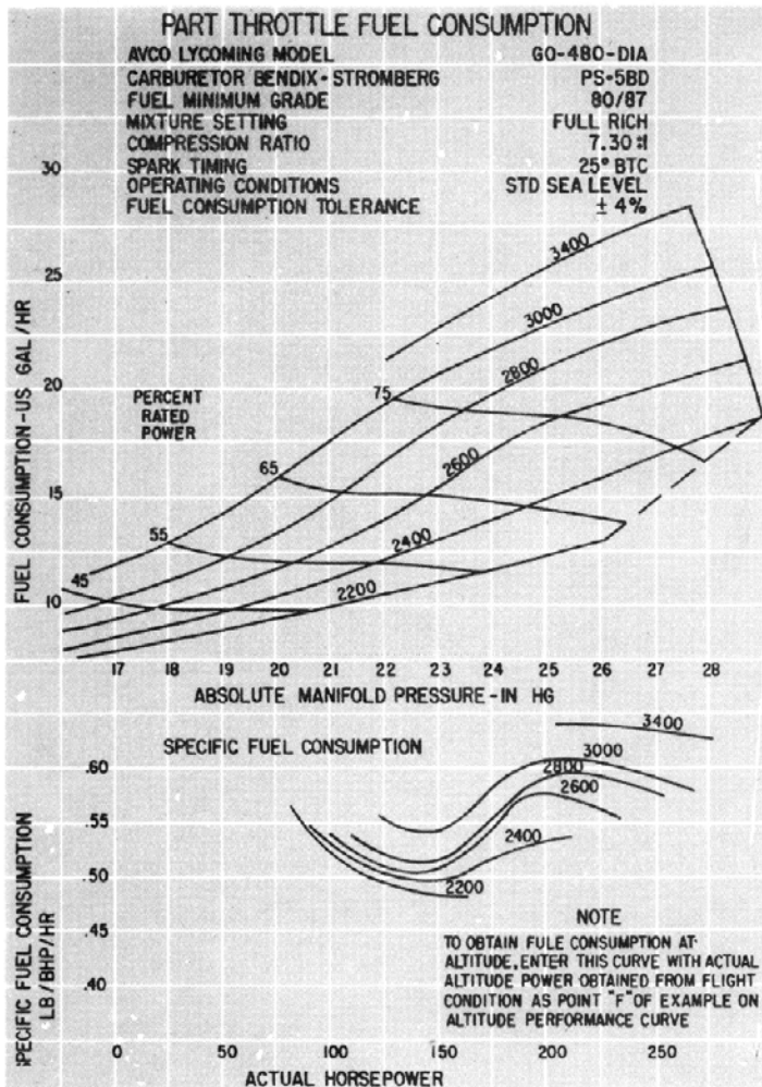
Figure 3-11. Part Throttle Fuel Consumption Curve - GO-480-D Series
