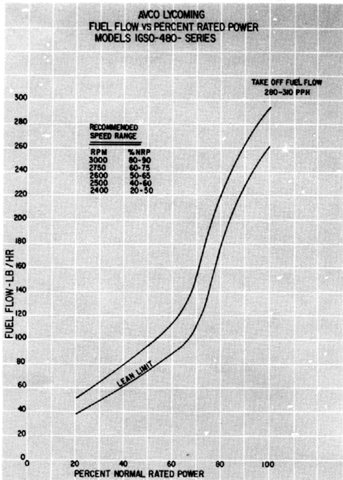
Figure 3-23. Fuel Flow vs Percent of Rated Power - IGSO-480-A1D6, -A1E6, -A1G6
