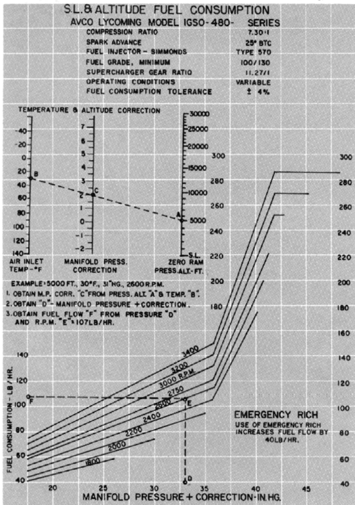
Figure 3-20. Sea Level and Altitude Fuel Consumption - IGSO-480-A1A6, -A1B6, -A1C6, -A1F3, -A1F6
