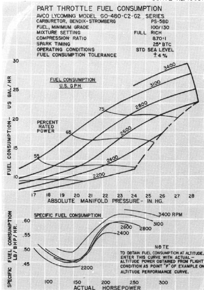
Figure 3-8. Part Throttle Fuel Consumption Curve - GO-480-C2, -G2 Series
