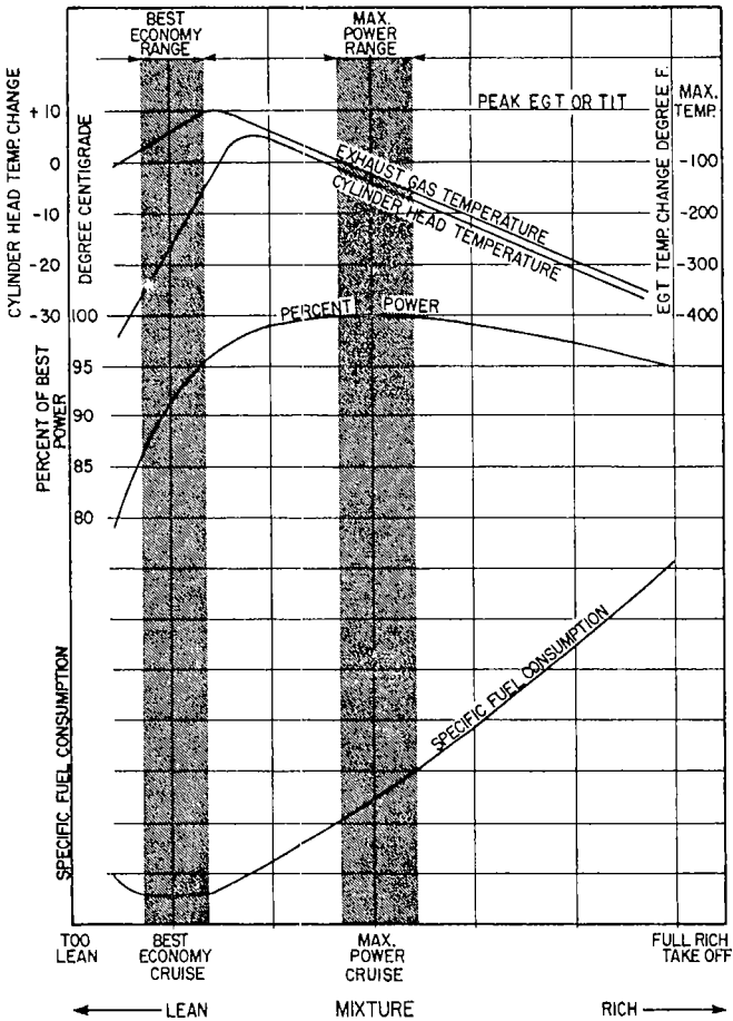
Figure 3-1. Representative Effect of Fuel/Air Ratio on Cylinder Head Temperature, Power and Specific Fuel Consumption at Constant RPM Cruise Range Operation
