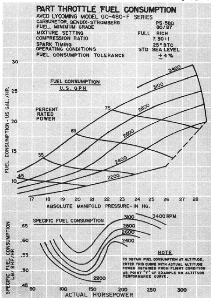
Figure 3-14. Part Throttle Fuel Consumption - GO-480-F Series
