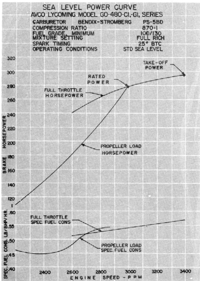
Figure 3-6. Sea Level Power Curve - GO-480-C1, -G1 Series
