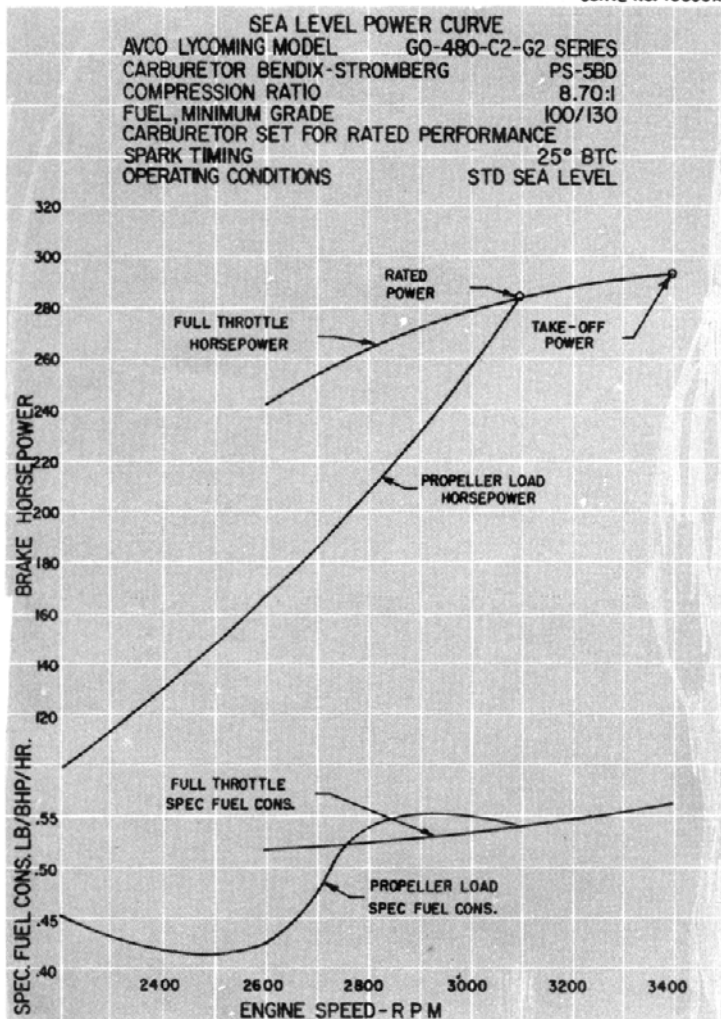
Figure 3-9. Sea Level Power Curve - GO-480-C2, -G2 Series
